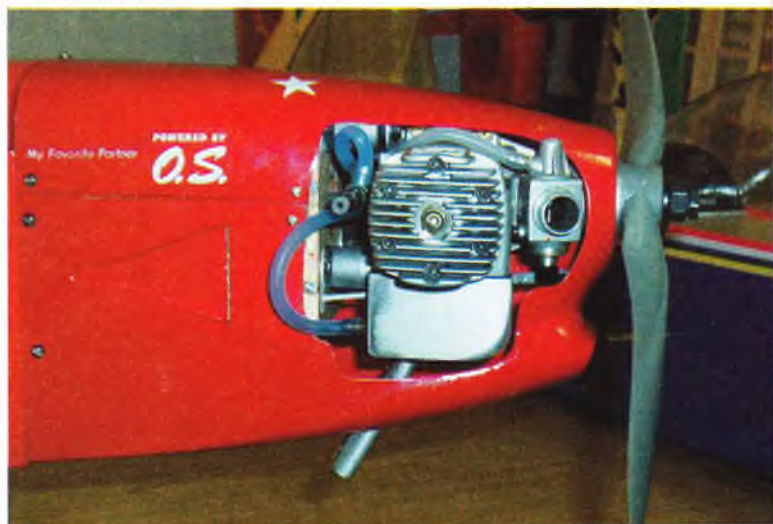
Motorinstallation.
