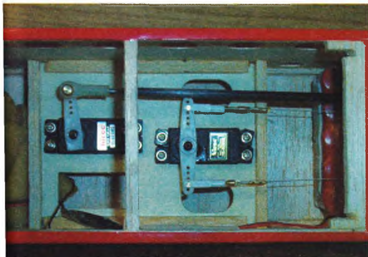
Servoinstallation.
