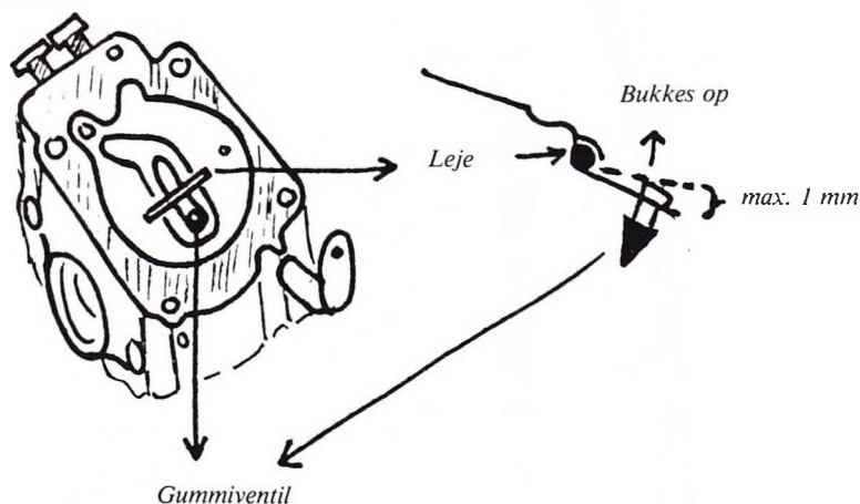
Fig. 1. Karburator adskilt.
