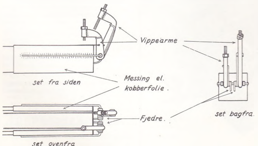
Skitse af tailplane-setting systemet i MESHACK.
