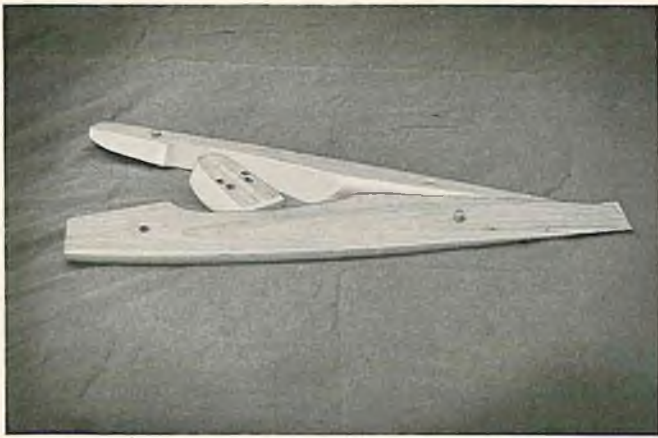
The carved "plugs" showing the dowels joining the 2 halves as a single unit while shaping. The chin radiator was also doweled under the nose to assure that the curves flowed between the three units.
