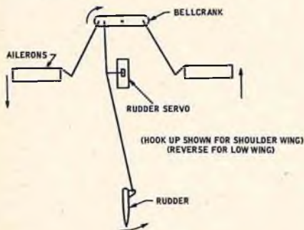
#3 RUDDER/AILERON CONNECTIONS
