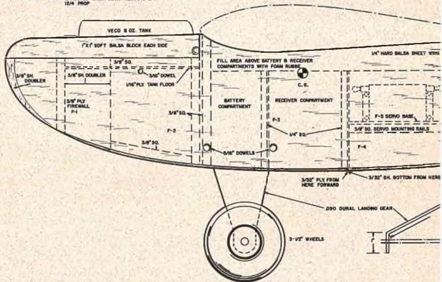
F-1 BLOCKS OMITTED FOR CLARITY
