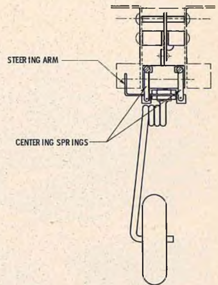
FRONT VIEW OF NOSE GEAR
