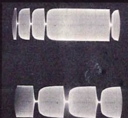
Collector of Q11. 200 us/div. 2 volts/div.
