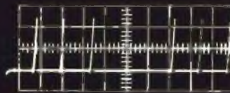
Base of Q10 1ms/div. 2 volts/div.
