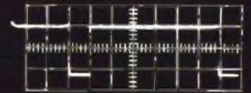
Collector of Q10. 200 us/div 2 volts/div.
