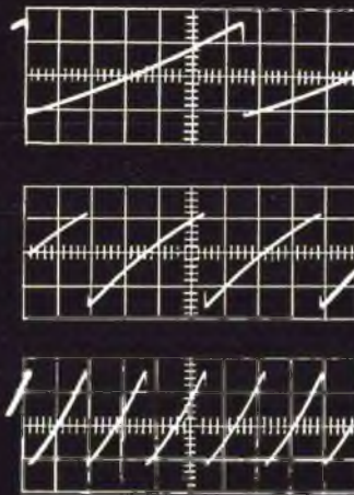
Output of pulse generator taken at point A showing effect of varying R23 and R30.
