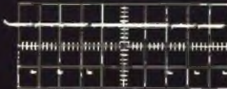
Collector of Q10. 1ms/div. 2 volts/div.
