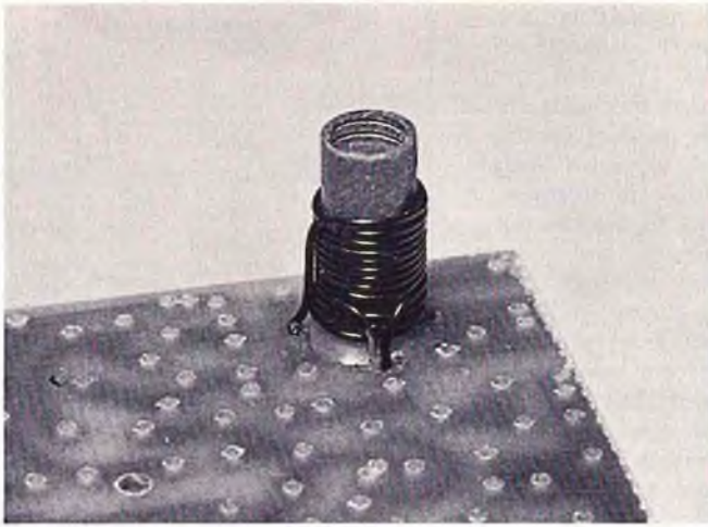
This photo clearly shows the winding and placement of leads for L1. First step in assembling receiver. Coil form is epoxied to P.C. Board — we used Hobby epoxy Glue.
