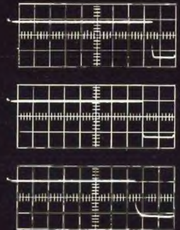
Collector of Q6-500 us/div. 2 volts/div. showing effect of stick movement.
