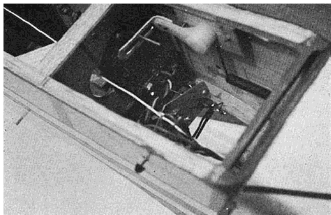
View of motor control, bellcrank, and sleeves adjustment tube, on engine control pushrod. Latter allows infinite adjustments.
