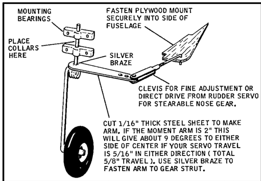
Gary Wedye of Alhambra, Calif. submitted this aid for straighter trike-geared tracking for Class I ships with fixed nose gear.
