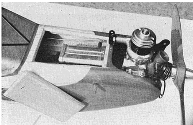
Engine control pushrod goes through firewall, then doubles back to loop through throttle arm. Note slant of hatch sides. Perfect #19 tank used.
