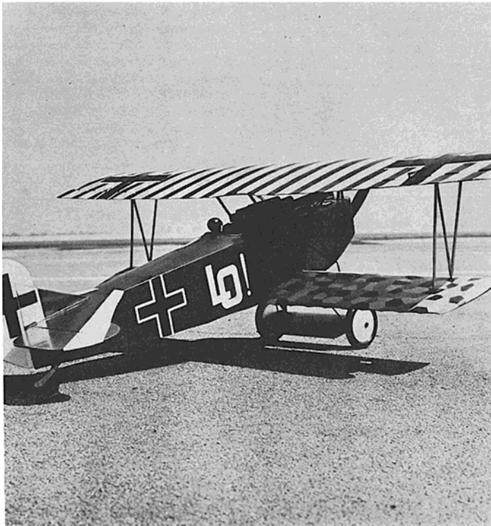
Another biplane — this time, F.A.S.T. Club member Chuck Coryell's World War I Fokker D-7, mistakenly attributed to the Williams brothers when it appeared in color on the January issue of R/C Modeler. Chuck's scale ship spans 57", uses a Supre Tigre .56 for power. Orbit reed equipment. Photo by Les McBrayer.
