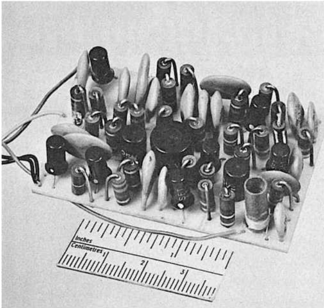
New superregen design concept outperforms superhets in interference areas.
