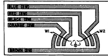
FIGURE 3. SWITCHING BOARD
