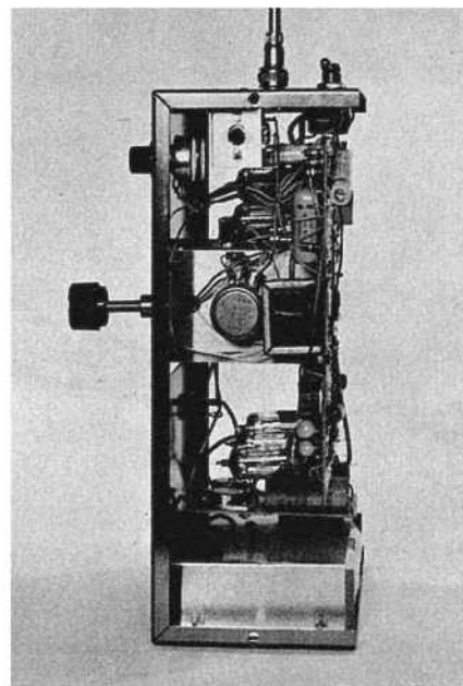
The airborne "21" system. Only change in RCM's test unit was an Ancco on throttle.
