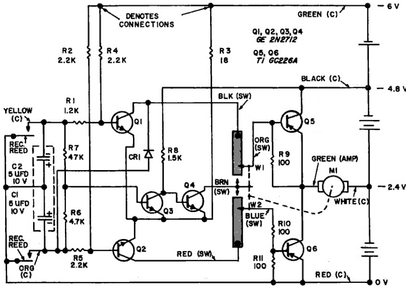
FIGURE 1. SCHEMATIC
