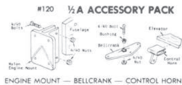
#120 1/2 A ACCESSORY PACK ENGINE MOUNT — BELLCRANK — CONTROL HORN
