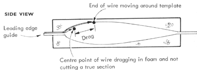
Figure 3 — Cutting wire too cold, or too slack
