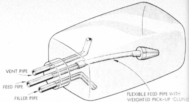
Figure 7: Clunk tank
