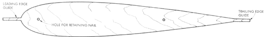
Figure 2 — Typical wing template. Use nails to fix to either end of foam blank. When cutting the foam, place the blank between wooden stops screwed to the workbench and then place a book or similar large heavy object on top of the blank to keep it firmly in place. You need both hands to operate the hot wire cutter.
