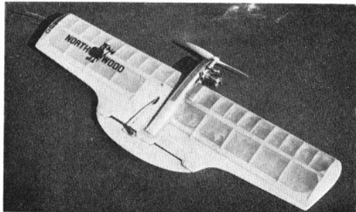
Pete Tribe developed his original Razor Blade until it looked like this (left) but still the basic layout remained, with \frac{3}{8} in thick section, \frac{1}{4} in sheet trailing edge and spruce spars. Mike Davis (right) simplified combat models with his Dominator - no spars, hefty leading edge and almost unbreakable when nylon covered.
