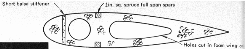
Figure 2 Typical 'foam' model and airfoil section.
