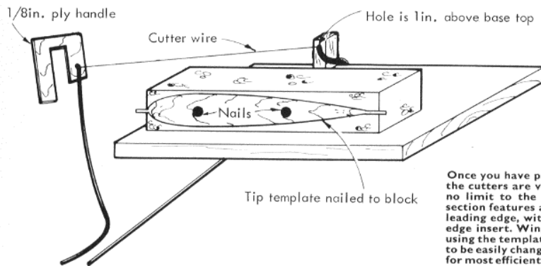
Figure 6 ▲ Using a special jig and cutter to form wing tips for combat models.
