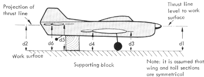
Figure 1 - Checking alignment
