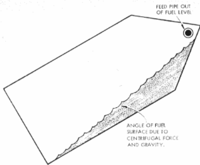
Figure 6: Engine starved of fuel (view from rear)
