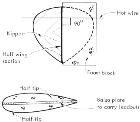
Figure 7 Using a 'kipper' to form elliptical tips
