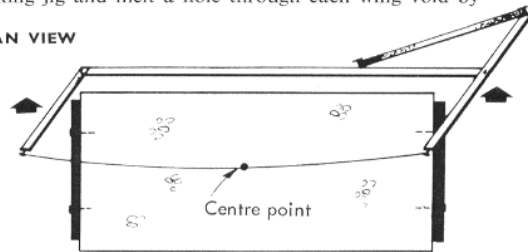
Figure 3 — Cutting wire too cold, or too slack
