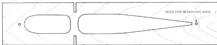
Figure 4 ▲ Template for cutting voids and surface spar slots. Use different templates at tip and centre to provide lighter tips if desired.
