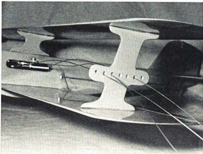
Lower right: Adjustable leadouts provide for windy or calm conditions. Moved forward line tension is less but speed is higher.
