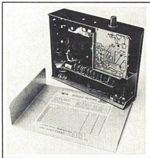
Top: In addition to the above parts, the Custom systems also include all servo trays, frequency flag, an excellent instruction manual, and plenty of servo output arms. Above: New Orbit single deck receiver. It now operates at full range between 4.8V down to 3.6V. A one-cell battery failure is not a guaranteed disaster as in the past. Left: New feature in the transmitter is the attached service record card. The technician who does the work also signs the card. This speeds service and assures quality work. Below: Workshop effort on the Intruder is finished—now for some flying.
