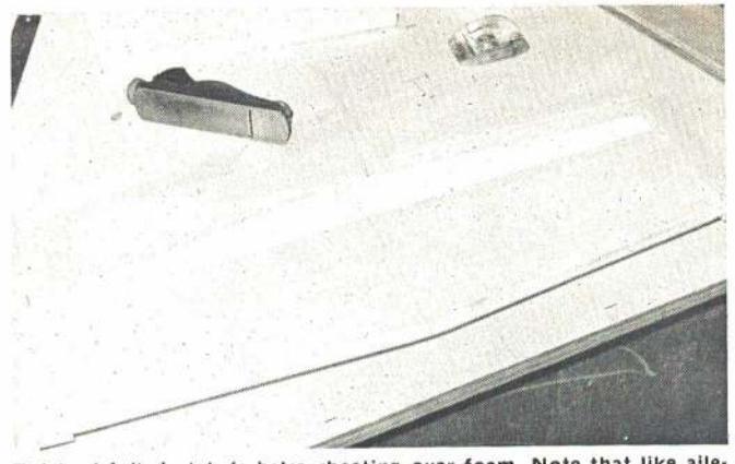
Thick airfoiled stab is balsa sheeting over foam. Note that like ailerons, elevators are foam cored. This guarantees airfoil continuity.
