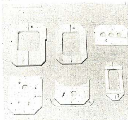
Very important to accurate modeling is use of centerlines throughout. Text describes in detail.
