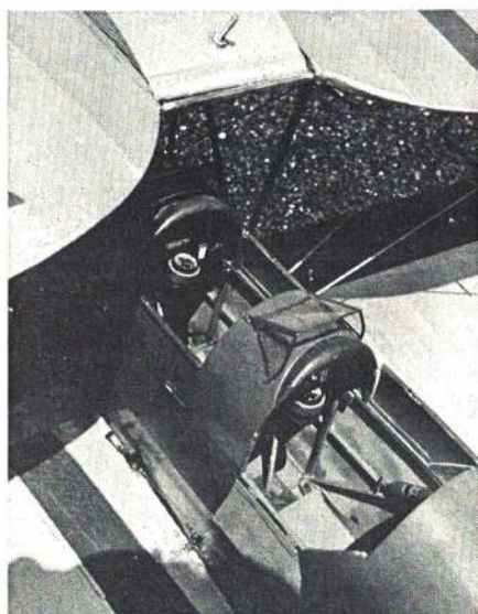
Left: Cockpit of Derek Goddard's deHavilland Tiger Moth. Highly detailed with long-rons and stringers visible, horizontal compasses, controls and fire extinguisher.
