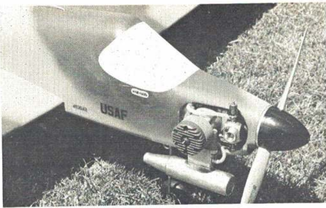
Neat and uncomplicated engine installation. Webra rests on Kraft-Hayes plastic mount.
