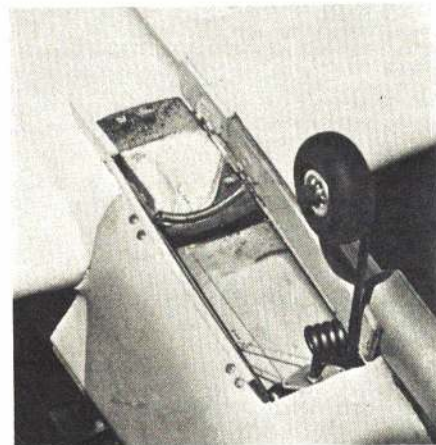
James Kubo's retract door mechanism. Note that the doors are segmented, and that a simple spring does the job. (photo by Jim Miura)
