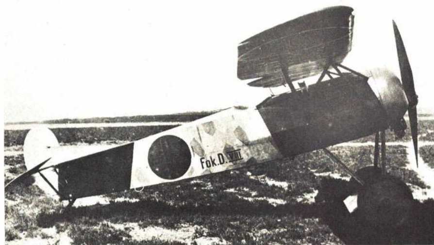
Since neither the guns nor factory markings are apparent, this is perhaps a production E. V awaiting upgrading to a D. VIII. On Nov. 1, 1918, 85 D. VIIIs were operational on the western front.
