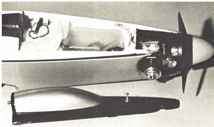
ABOVE: The one-piece hatch is removed to show the Sullivan two-oz. tank installation. Airborne batteries are located, in foam, just aft of the tank. RIGHT: The Kirn-Kraft needle valve ensures peak setting for the Cox Tee Dee 049. Maximum performance, as with the 60-sized jobs, requires a screaming engine. BELOW: The sub-rudder is an aerodynamic necessity, but it also serves as a landing skid. The same holds true for the raked-down wing tips, which are the author's trademark.
