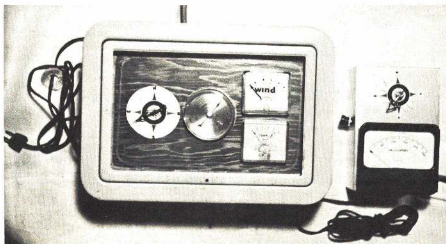
ABOVE: Cut out a hole for the milliammeter in a metal case (this one from Ace R/C). Three small holes are for slave servo, to indicate wind direction. BELOW: Two completed wind direction and velocity monitoring units. Larger unit houses a barometer, as well as an additional meter for a future project. This case is a discarded "exit" sign box.
