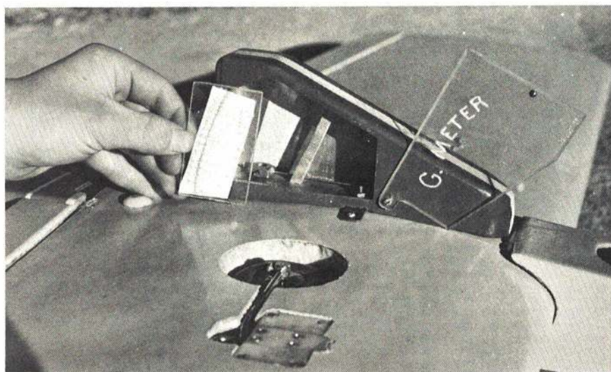
The calibrator is a scale which reads multiples of the original weight of the arm. The scribe marks on the paper are compared to the calibrator to give interpretive readings.
