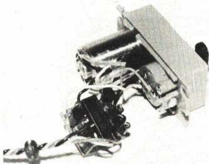
Texas Instruments worked out Kraft-designed amplifier IC with bridge circuit amplifier capable of safe operation at 3.6V.
