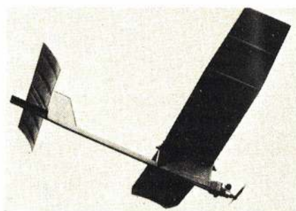
Side/bottom view of a Mini-Rod (February 1969 AAM) under full DT coming to earth.
