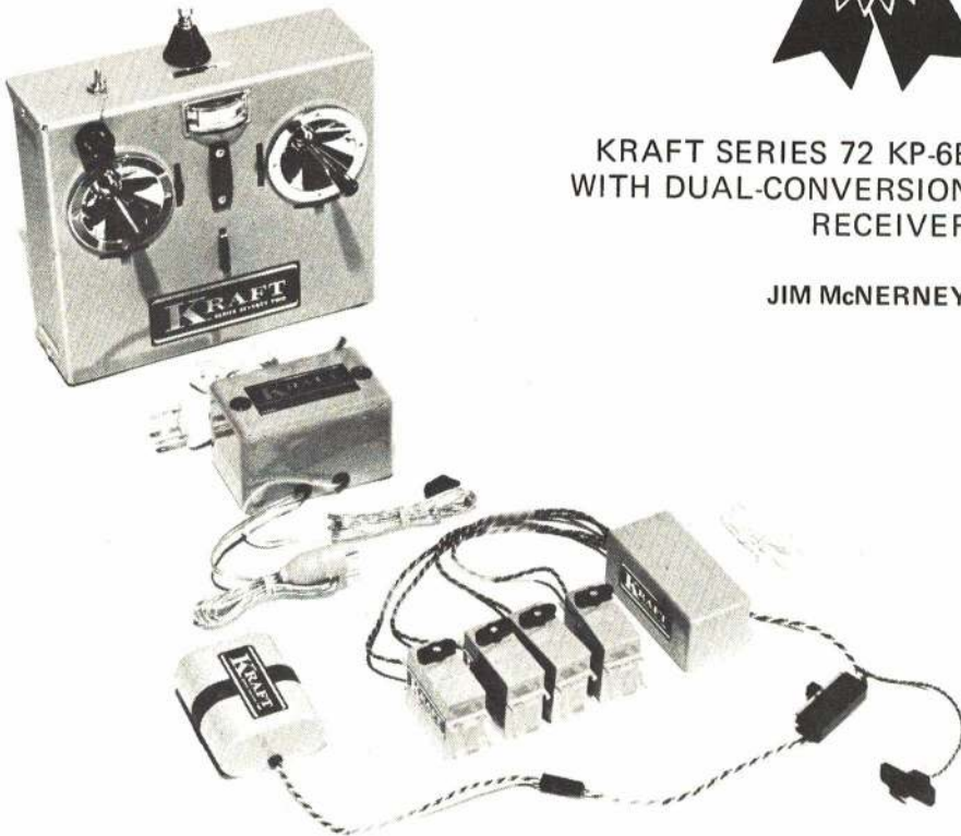
Above: Noticeable here is large 550 mah battery pack. Cells are new super-reliable high charge rate types.
