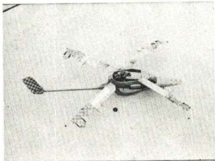
In free flight, Dr. Lee Taylor flew this familiar model. Separate blade sections provide cyclic and collective pitch control.
