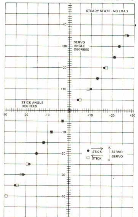
FIGURE 1 KRAFT SERIES SEVENTY-TWO KP-6B 8-15-72
