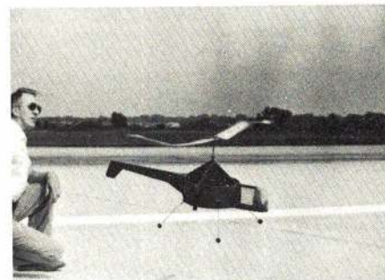
Glen Lee's large 15-powered FF model has low disc loading and so its sink rate in autorotation is very slow. Engine is on the main shaft for torque reaction drive but located below and inside the fuselage.
