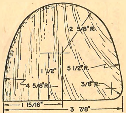
MAKE STABILIZER & RUDDER OF 1/16".
