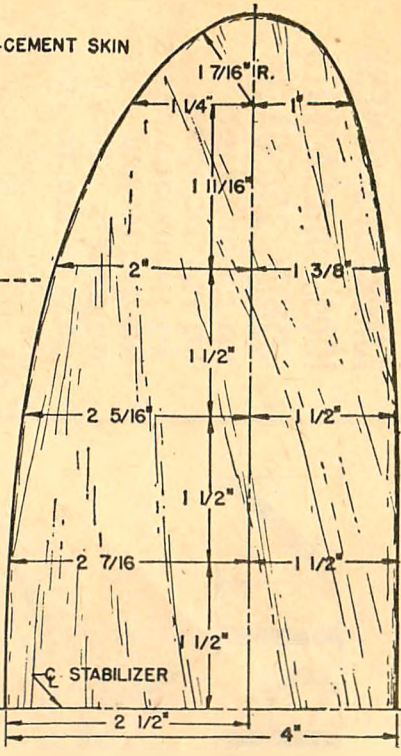
MAKE STABILIZER & RUDDER OF 1/16".
