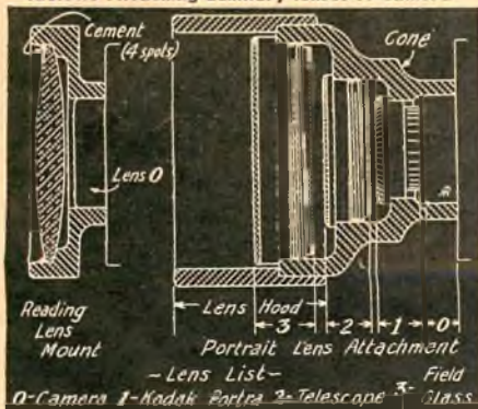
(Above) Parallax correcting mount (Below) Attaching auxiliary lenses to camera
