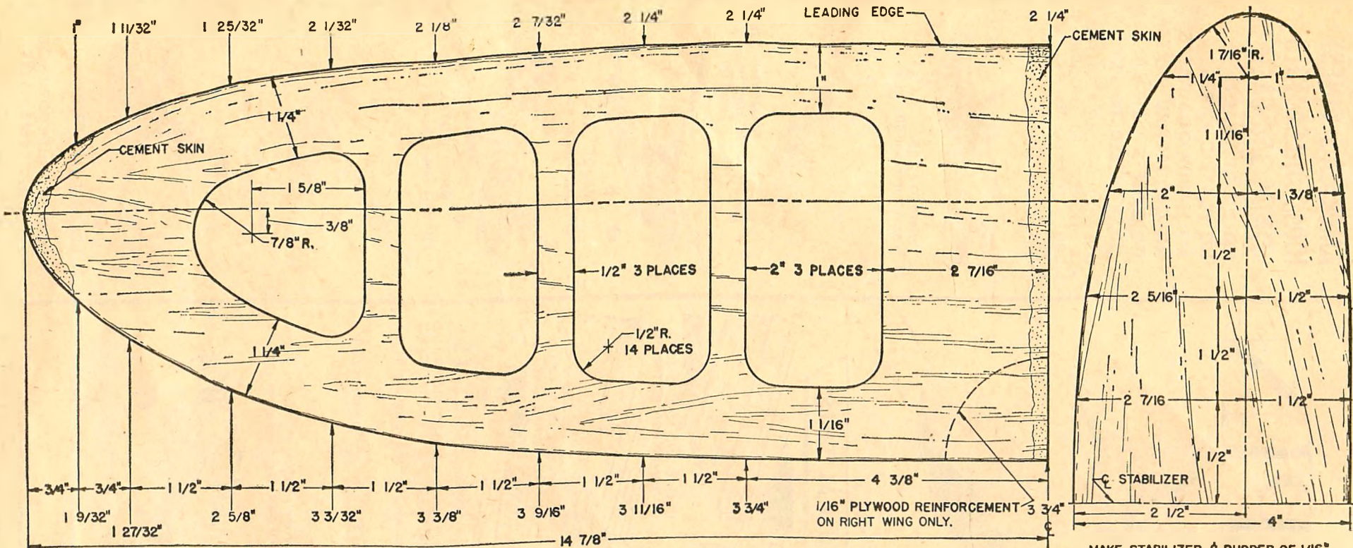
WING & TAIL SURFACES HALF SCALE
