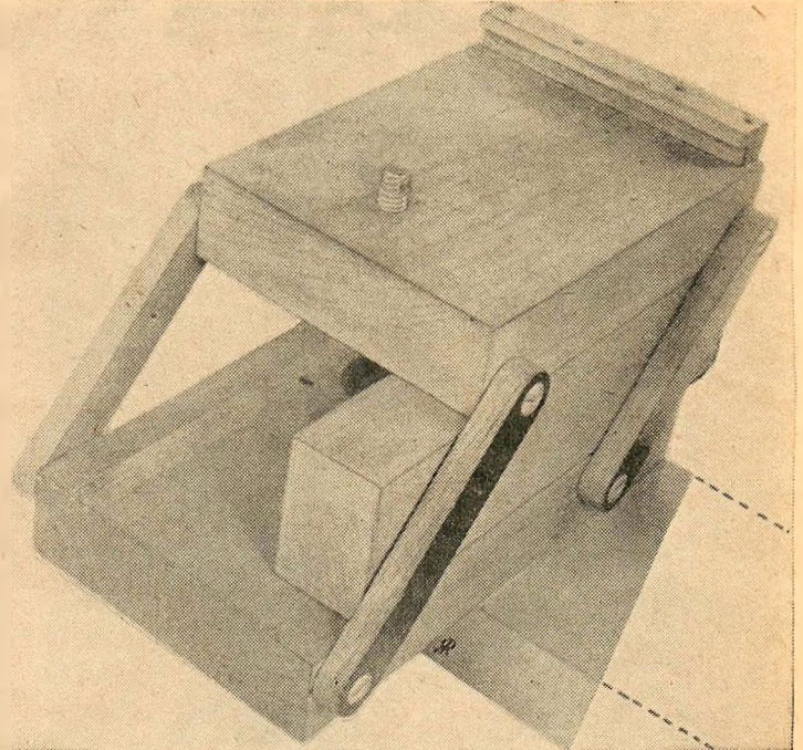
Linkage in "shooting" position with filler block in place
