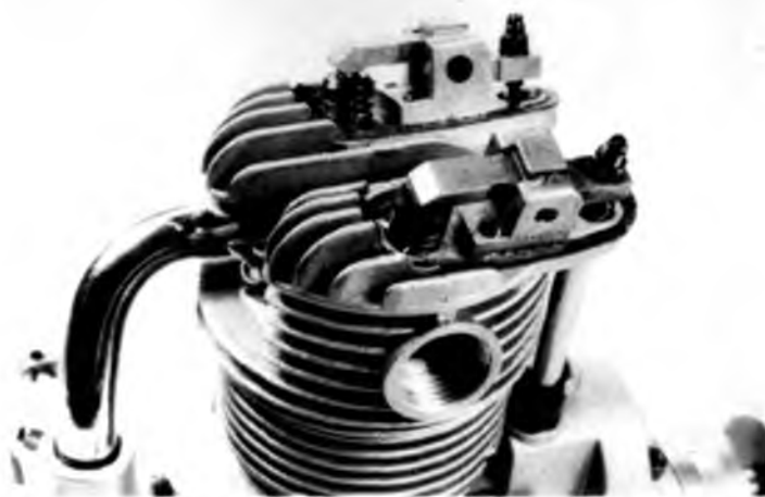
Above: Inclined valves are Saito tradition. Rocker covers removed to show neat valve gear. Right: Saito carburetor has automatic fuel metering via tapered groove in end of throttle barrel.
