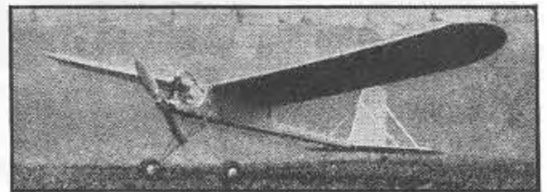
Mel Anderson's stick gas job that weighs only 14 1/2 ounces. The wing span is 46 1/2". It is easy to transport because of its small size. Pict. No. 9
