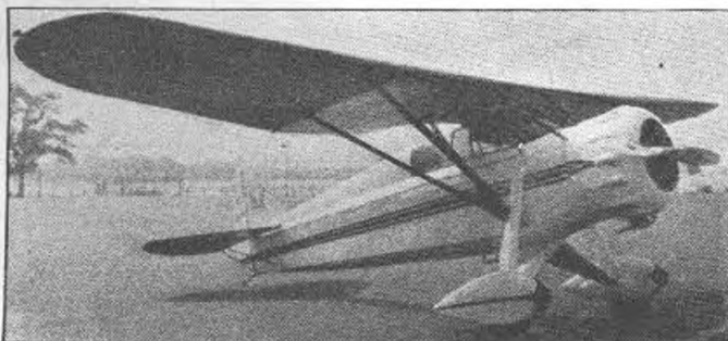
The Davis D1-W De Luxe sportplane powered with a Warner Super-Scarab 145 hp. engine (Tenety)
