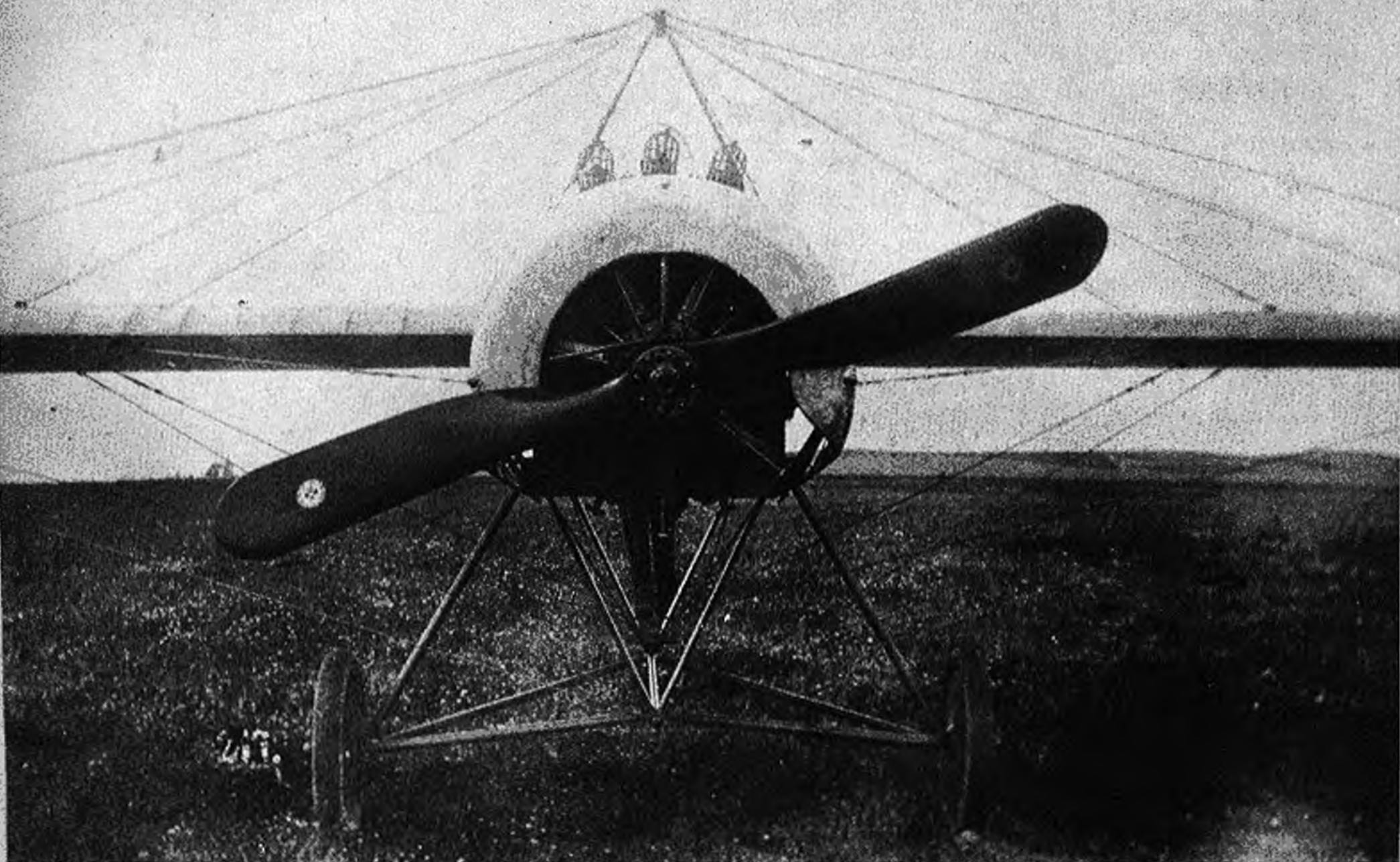
On the strength of the initial advantage of the Fokker E-1 and its synchronized guns the Germans built this special three-gun job for Max Immelmann.
