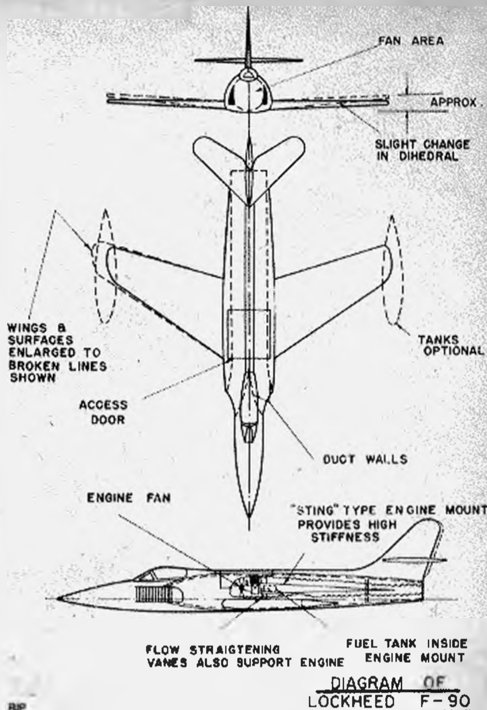
Three-view drawing of a proved Lockheed. Note engine, fan location. Below—Close-up of an .049 Wasp installation in a Cutlass. Note side intake screens. Bottle cap is handy starter. K & B and fan, also shown.
