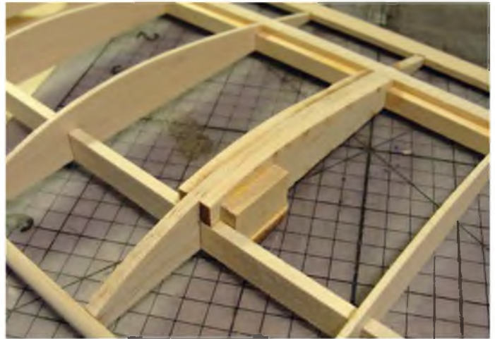
Despite the retro fitted aileron, this is a top wing panel. Note the strut socket and the hard point Alby fitted for diagonal strut attachment.
