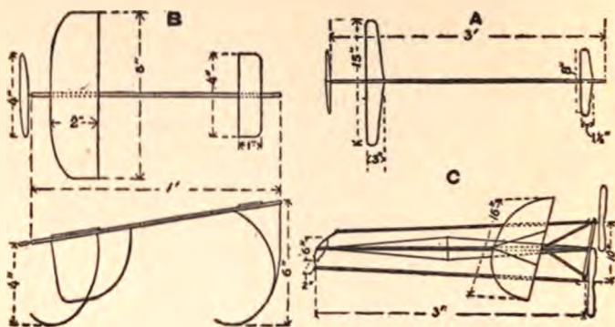
A—THE FAMOUS "ONE OUNCE." B—A SMALL EXPERIMENTAL MODEL. C—A MODIFIED BURGESS WEBB MODEL.
